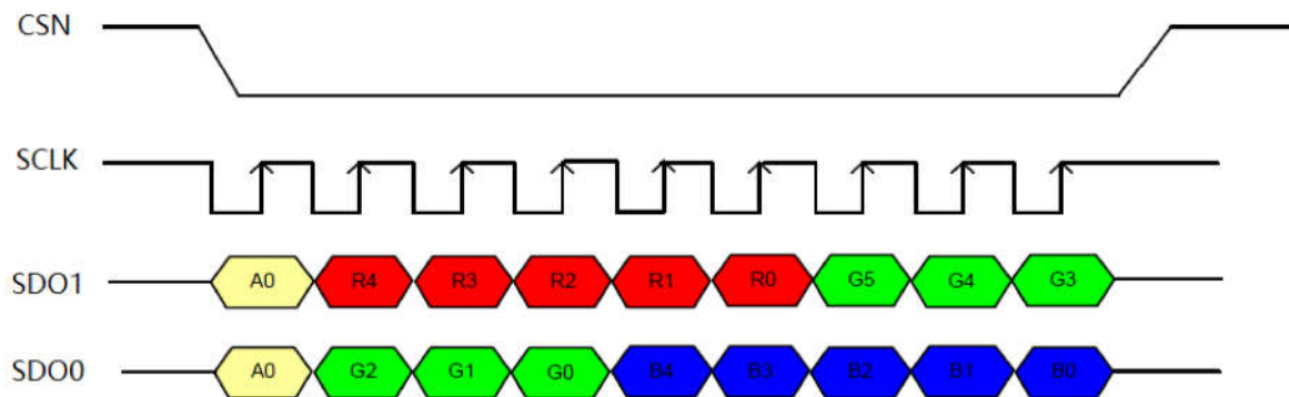
Figure 10-17 RGB666 Pixel Transition
