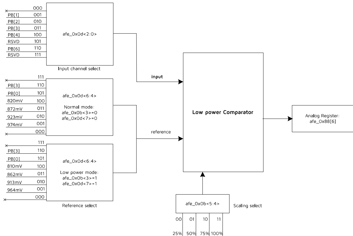
Figure 15-1 Block Diagram of Low Power Comparator
