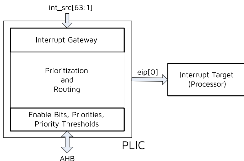
Figure 9-1 Block Diagram of PLIC
