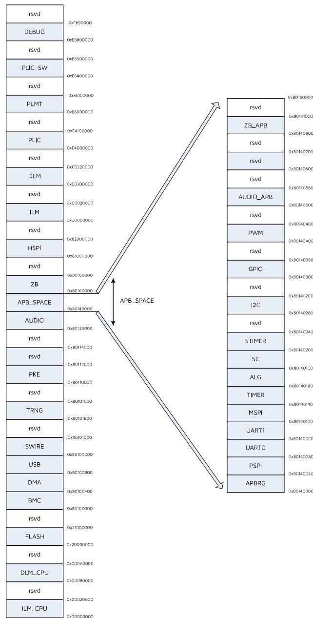
Figure 4-1 Memory Map
