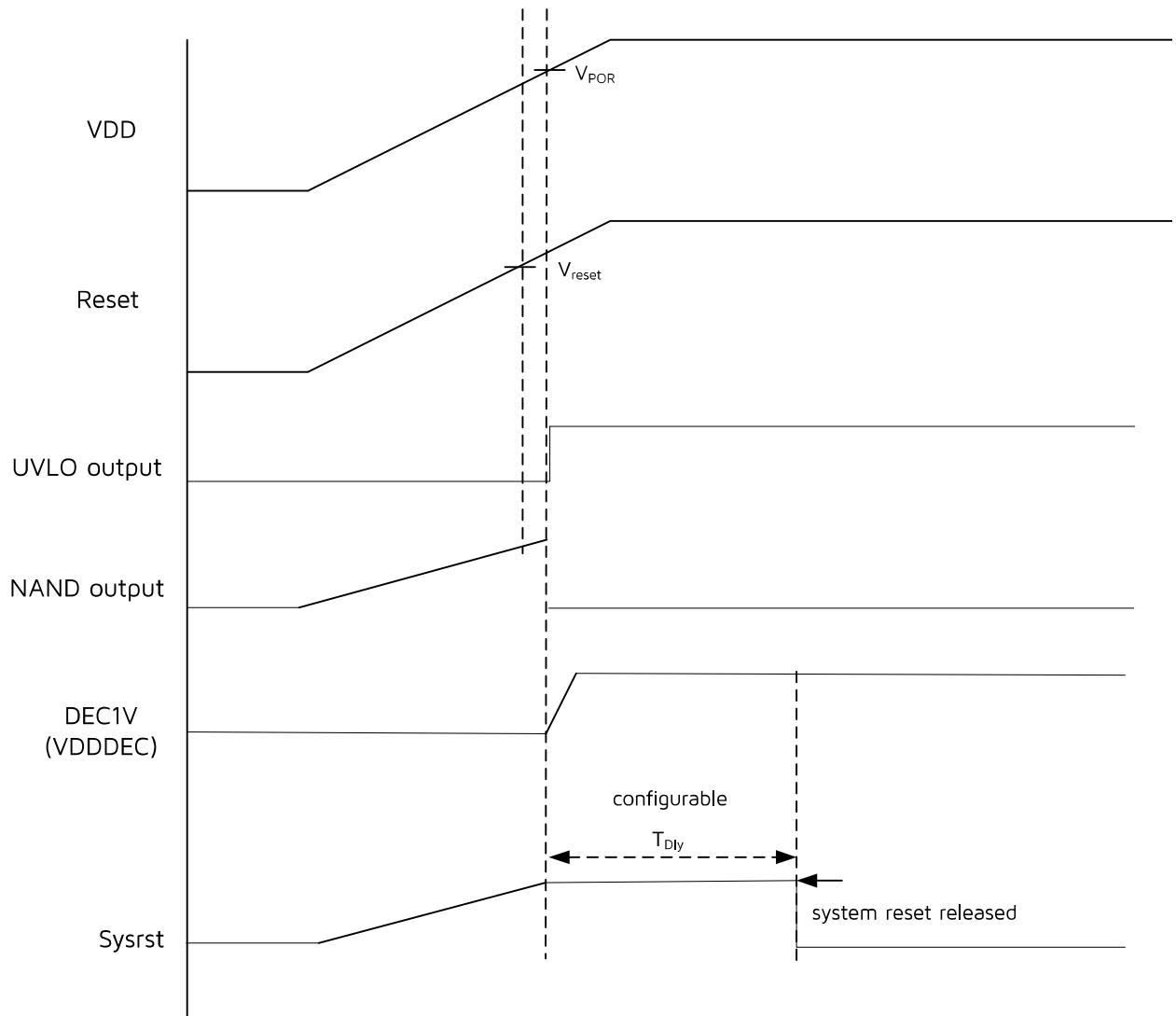
Figure 4-3 Initial Power-up Sequence
