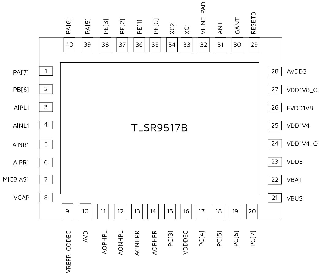
Figure 1-4 Pin Assignment of TLSR9517B
