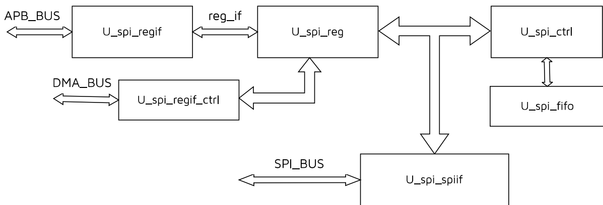
Figure 10-19 PSPI Diagram
