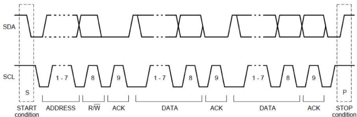
Figure 10-3 I2C Timing
