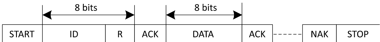
Figure 10-6 Write Format in Slave Mode
