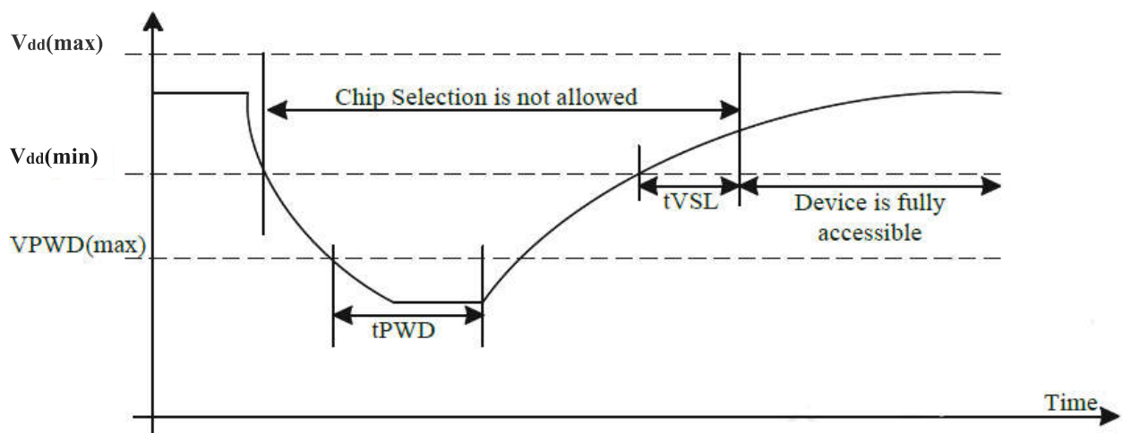
Figure 2-1 Power down-up Timing
