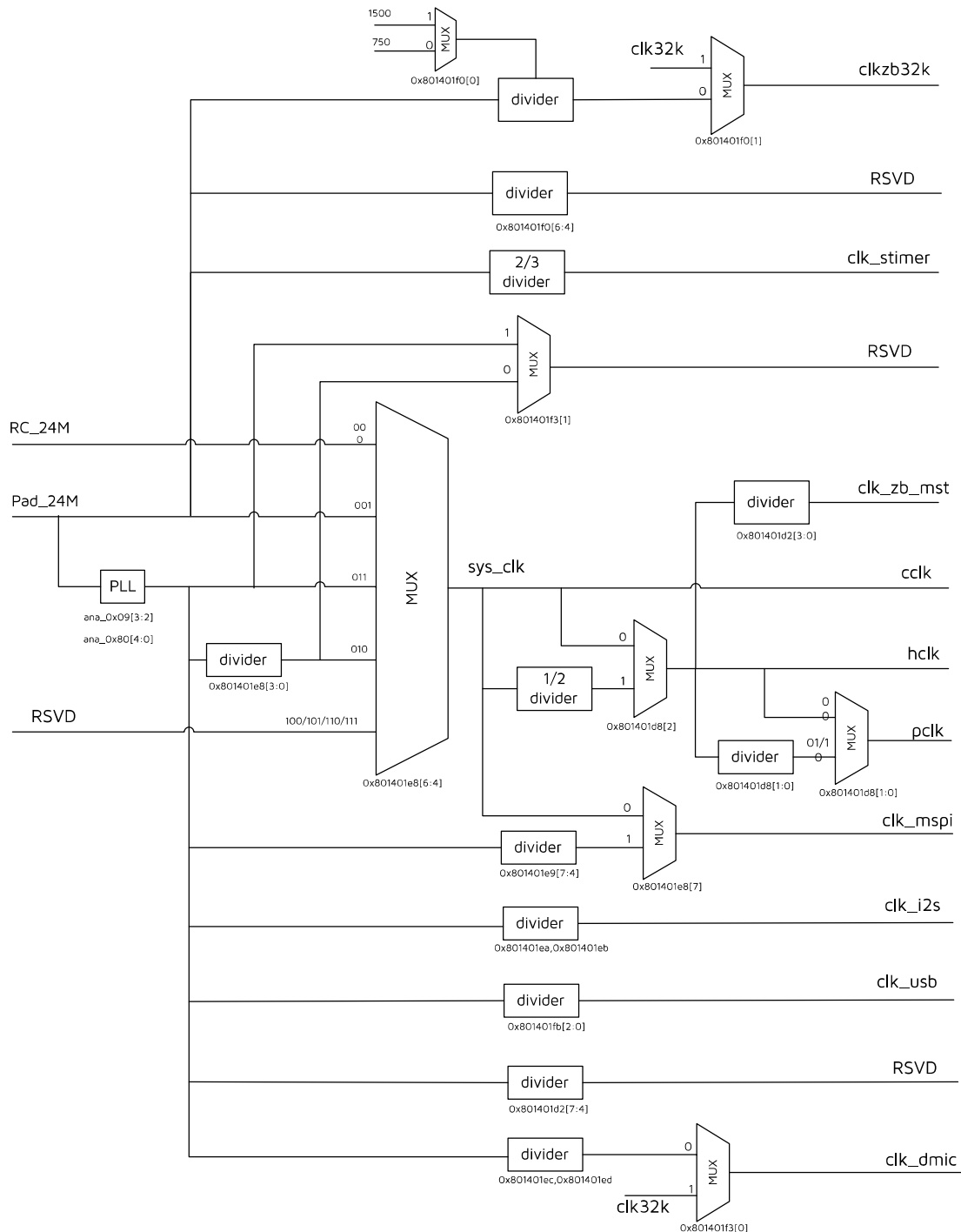
Figure 7-1 Clock Source
