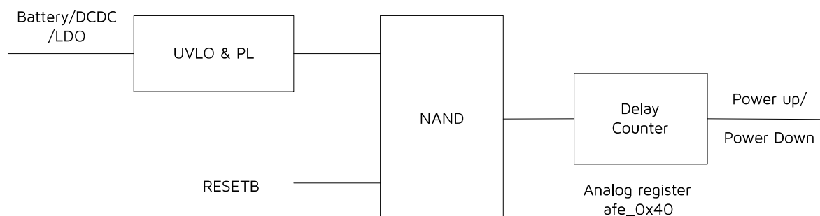
Figure 4-2 Control Logic of Power up/down
