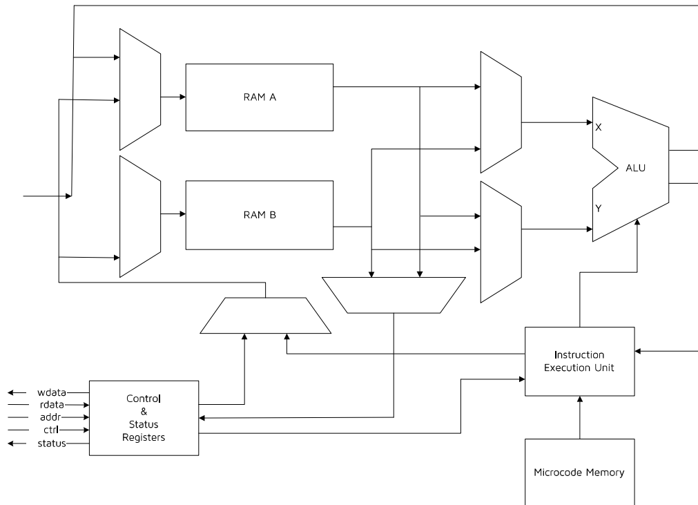
Figure 17-1 Block Diagram of PKE SP Module
