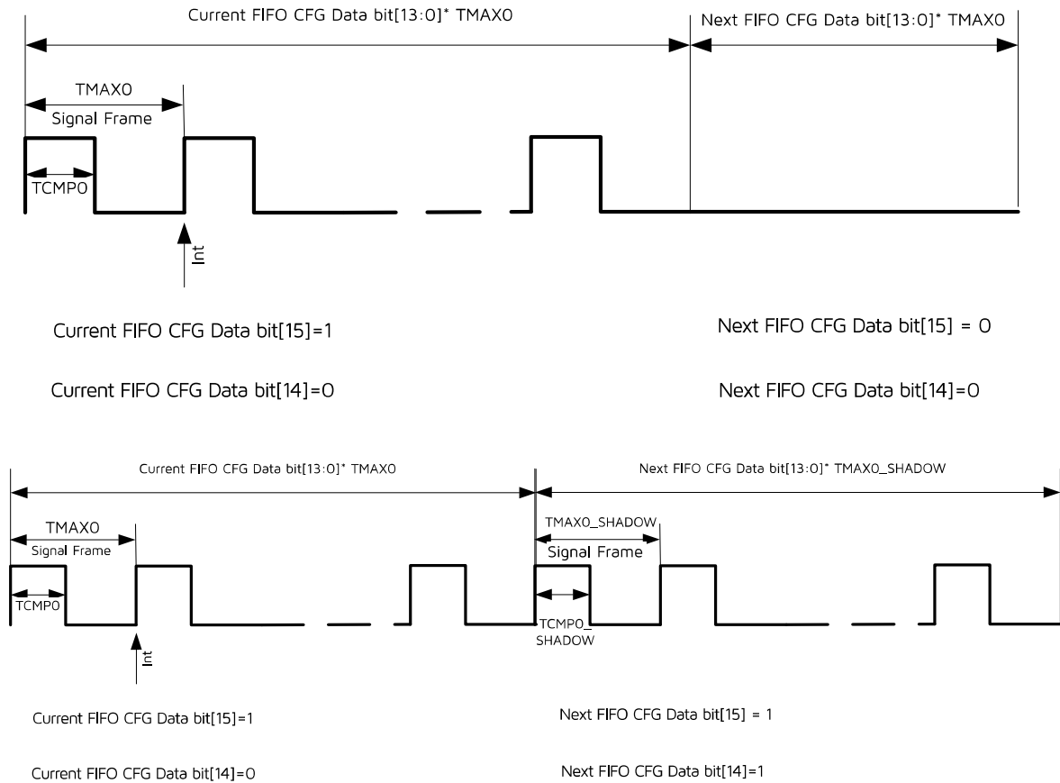
Figure 11-6 IR Format Examples
