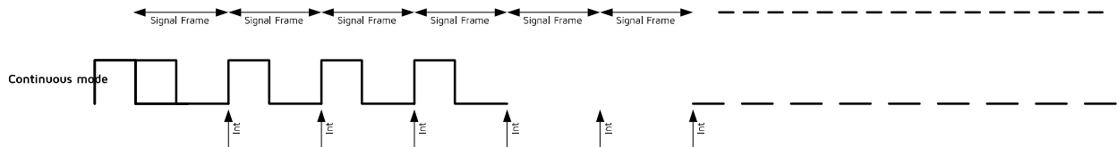
Figure 11-3 Continuous Mode
