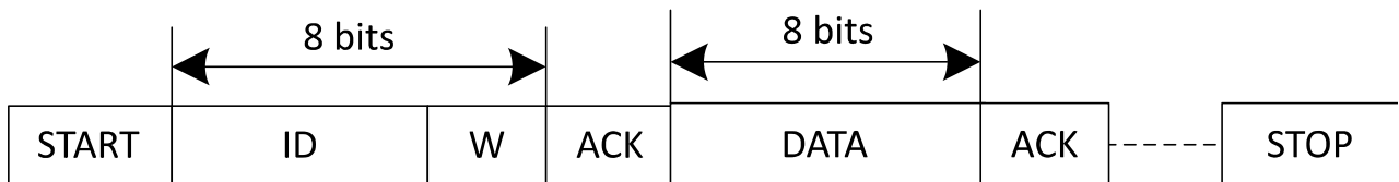
Figure 10-6 Write Format in Slave Mode
