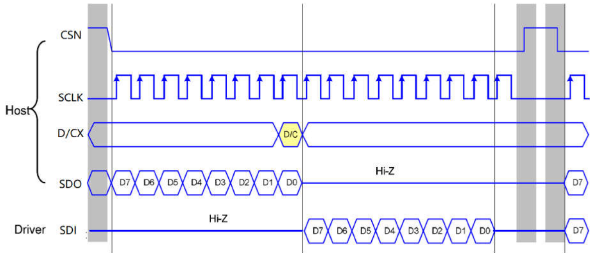
Figure 10-14 4-Line Read Sequence
