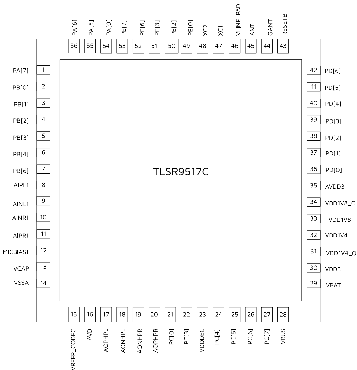
Figure 1-5 Pin Assignment of TLSR9517C
