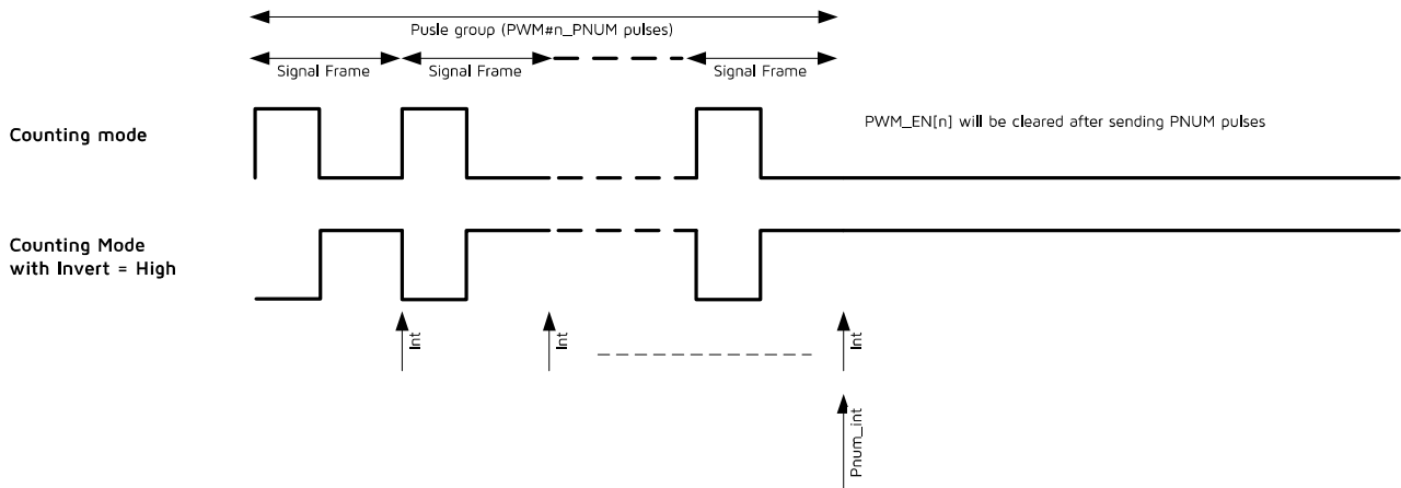
Figure 11-4 Counting Mode (n=0)
