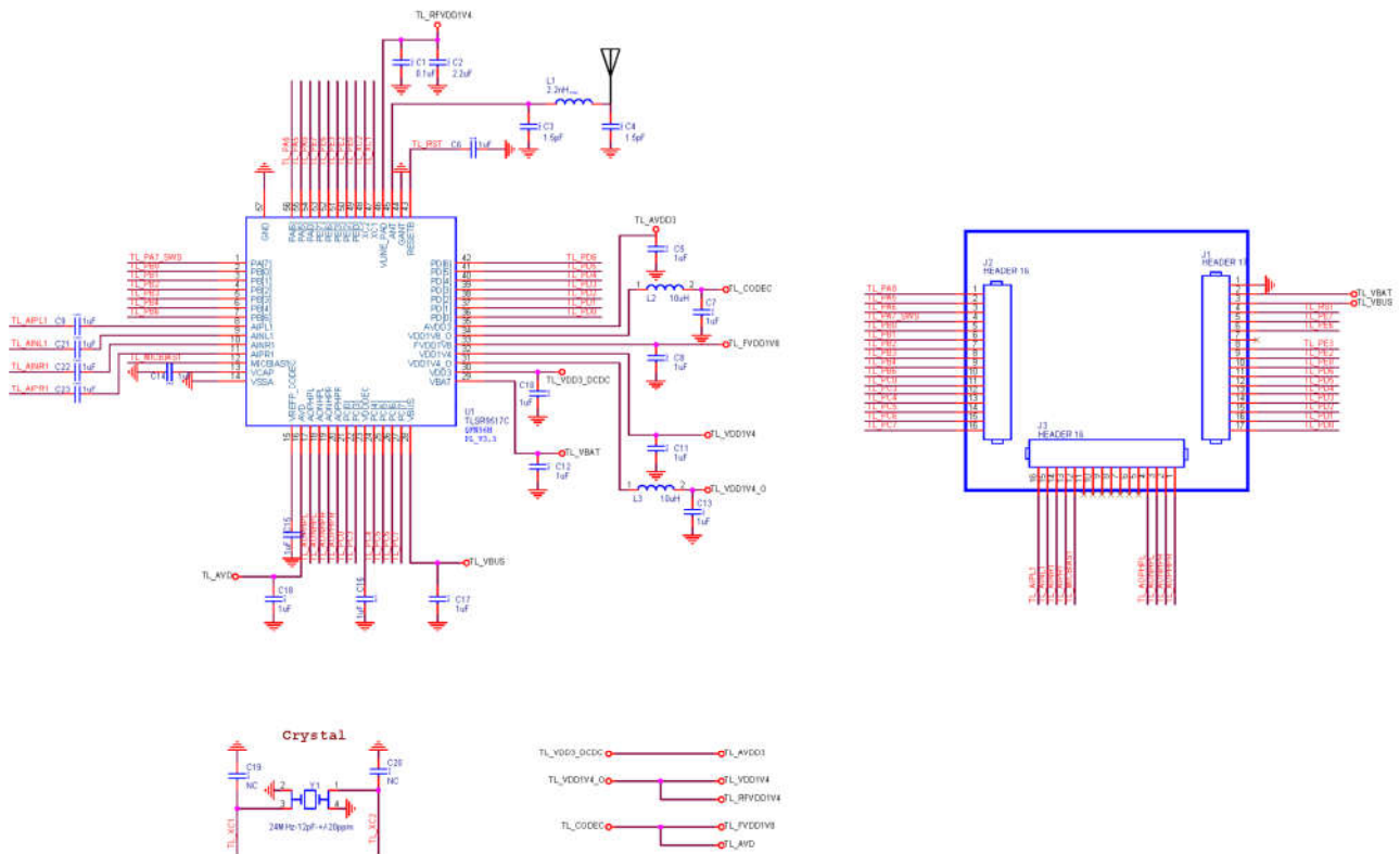
Figure 3-2 Schematic of TLSR9517C
