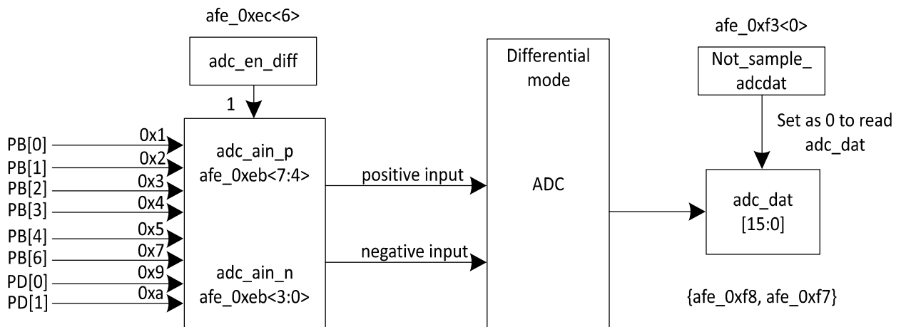
Figure 13-1 ADC Diagram For TLSR9517
