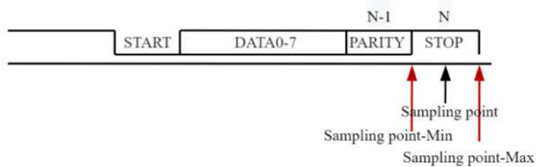
Figure 10-23 UART Protocol Formats and Sampling Point
