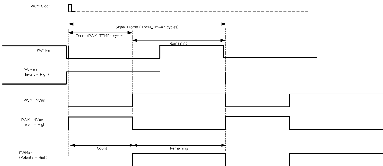
Figure 11-2 PWM Output Waveform Chart
