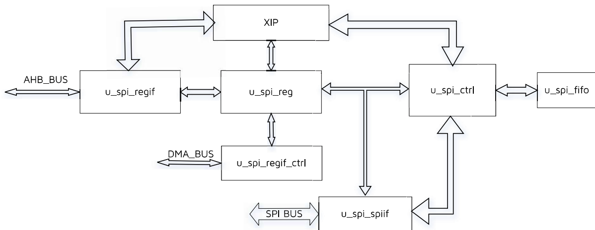
Figure 10-8 HSPI Diagram
