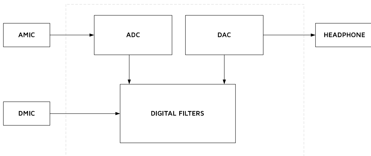
Figure 5-1 Audio CODEC
